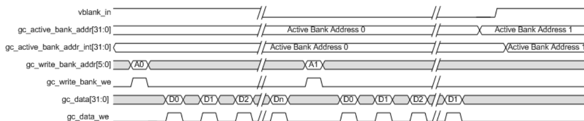
Figure 10: Graphics Controller Host Interface Timing
