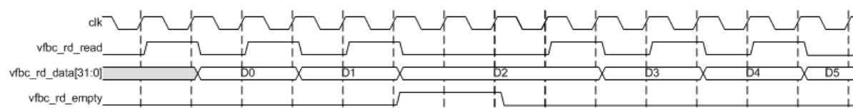
Figure 7: Read FIFO Interface Timing
