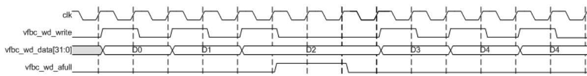
Figure 8: Write FIFO Interface Timing
