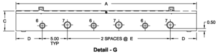
Detail - G
