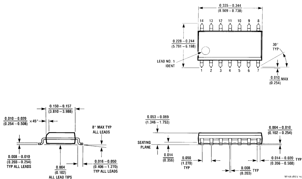
14-Lead Molded Small Outline Package, JEDEC Order Number 74LVX14M or 74LVX14MX NS Package Number M14A
