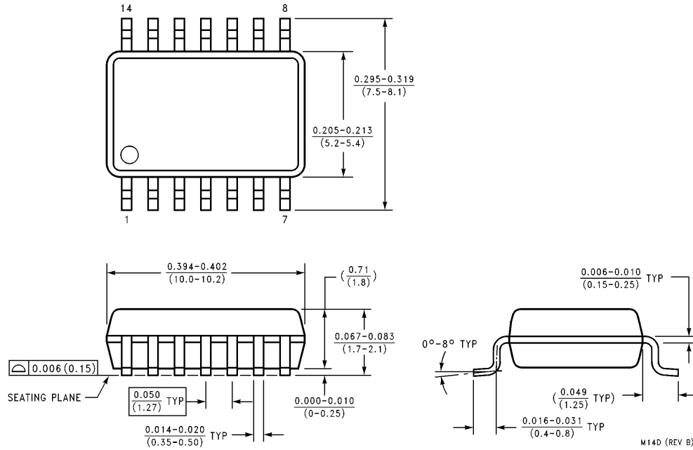
14-Lead Small Outline Package EIAJ (SJ) Order Number 74LVX14SJ or 74LVX14SJX NS Package Number M14D
