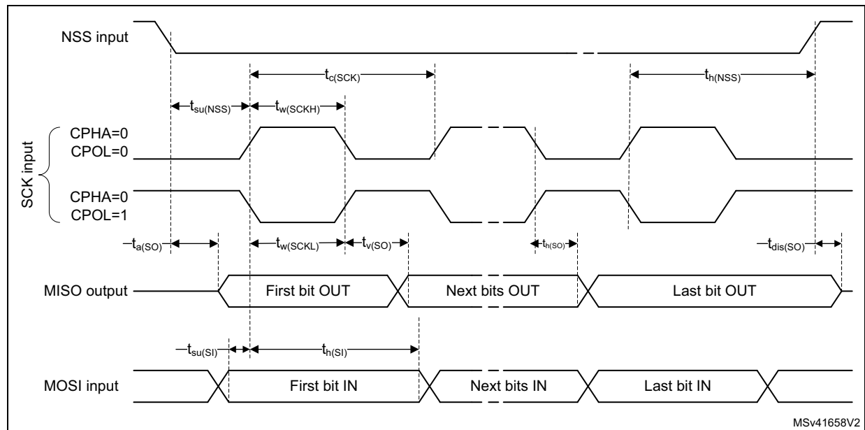
Figure 20. SPI timing diagram - slave mode and CPHA = 0
