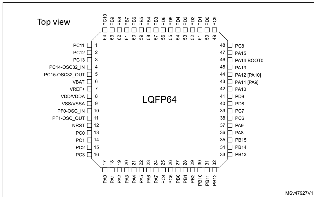
Figure 5. STM32G070RxT LQFP64 pinout
