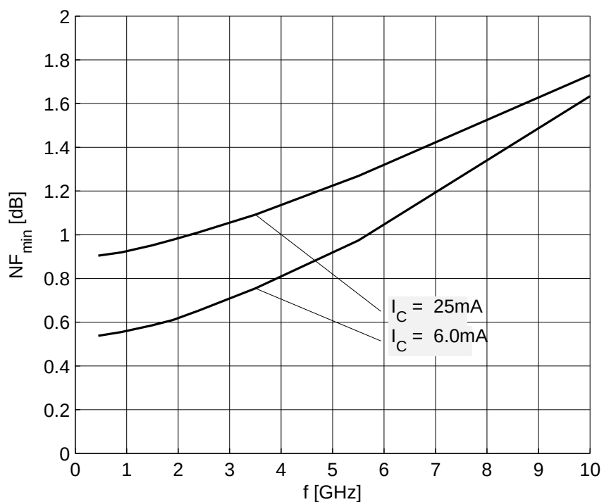
Figure 5-18 Noise Figure NF_{\min} = f(f) , V_{CE} = 3\text{ V} , I_C = 6 / 25\text{ mA} , Z_S = Z_{\text{opt}}
