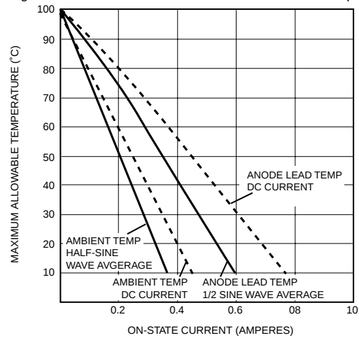
Figure 10. On-State Current vs. Maximum Allowable Temperature
