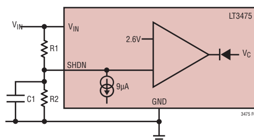
Figure 2. Undervoltage Lockout
