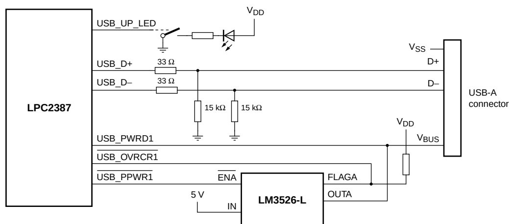
Fig 20. LPC2387 USB host port configuration
