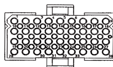
36 contacts AWG 16
