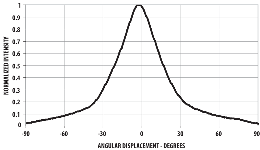
Figure 5. Radiation Pattern
