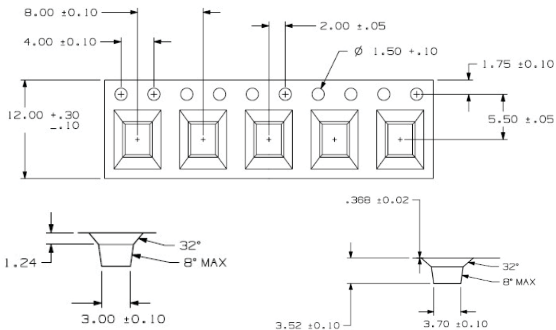
Figure 11. Tape Dimensions
