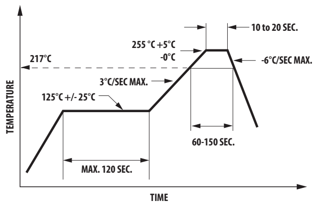
Figure 8b. Recommended Pb-free Reflow Soldering Profile.
