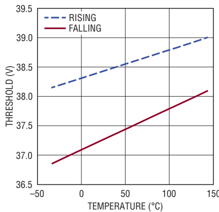
Overvoltage Lockout
