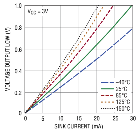
RST, PFO Voltage Output Low vs Sink Current
