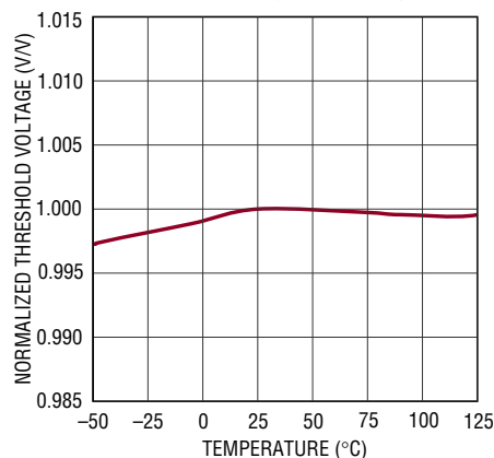
Normalized Reset and Power-Fail Threshold Voltages vs Temperature
