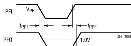
Power-Fail Timing
