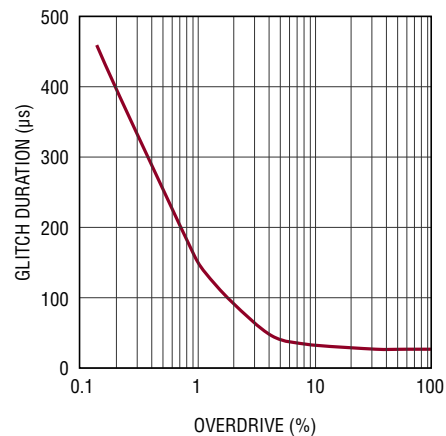
Allowable Glitch Duration vs Overdrive
