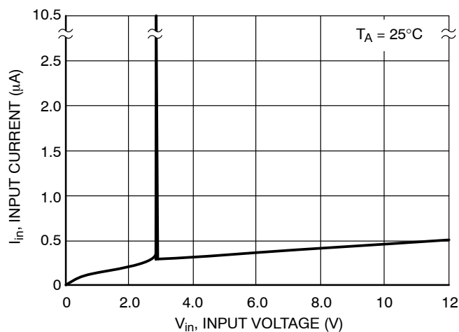
Figure 4. NCP302/3 Series 2.7 V Input Current vs. Input Voltage
