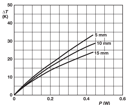
NFR25 Temperature rise ( \Delta T ) at the lead end (soldering point) as a function of dissipated power at various lead lengths after mounting
