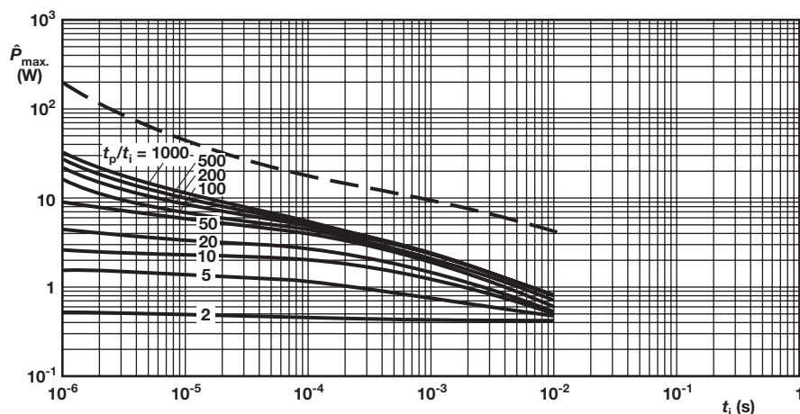
NFR25 Pulse on a regular basis; maximum permissible peak pulse power ( \hat{P}_{\max.} ) as a function of pulse duration ( t_i ), 0.22 \Omega \leq R \leq 15 \Omega
