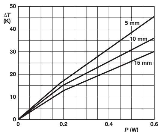
NFR25H Temperature rise ( \Delta T ) at the lead end (soldering point) as a function of dissipated power at various lead lengths after mounting
