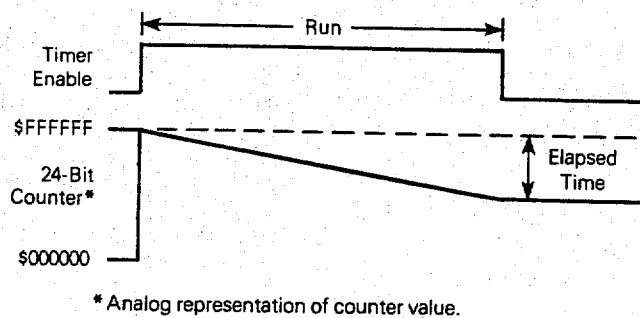
Figure 5-4. Elapsed Time Measurement Example
