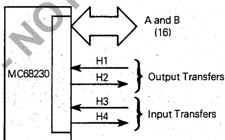
Figure 1-2. Port Mode Layout (Sheet 2 of 2)
