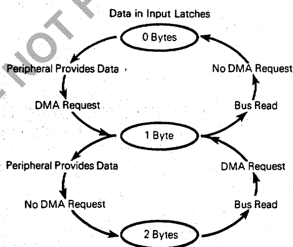
Figure 2-4. \overline{\text{DMAREQ}} Associated with Input Transfers
