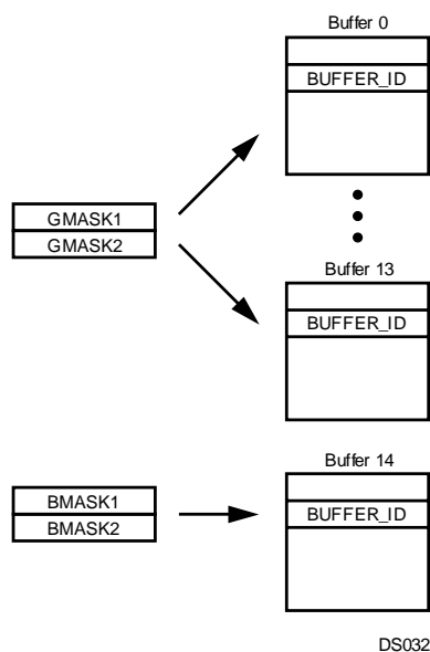
Figure 22-15. Acceptance Filtering
