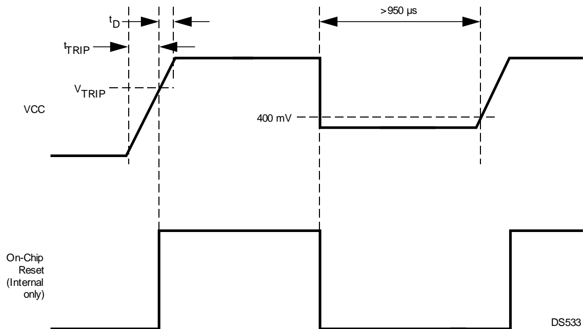
Figure 36-4. Power-On Reset
