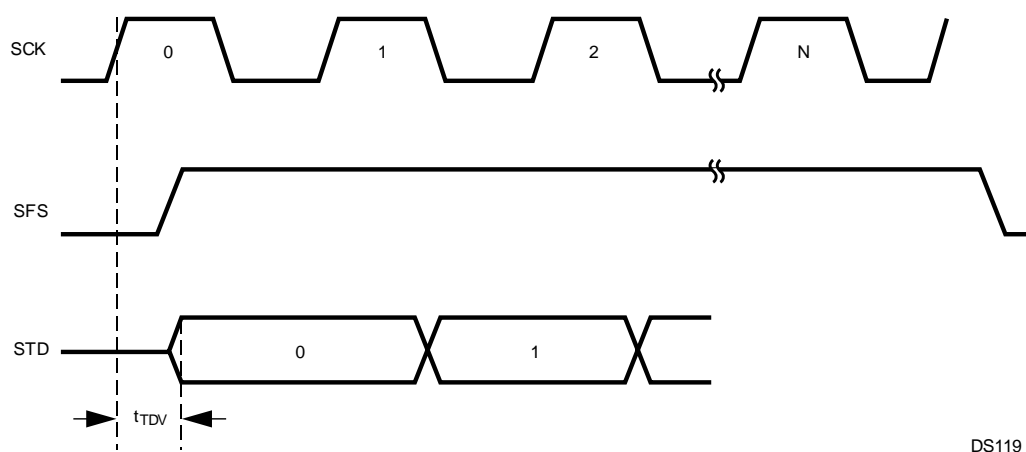
Figure 36-12. Transmit Timing, Long Frame Sync
