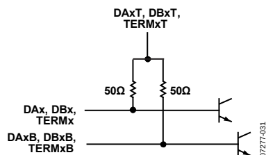
Figure 31. Input Termination Schematic Diagram
