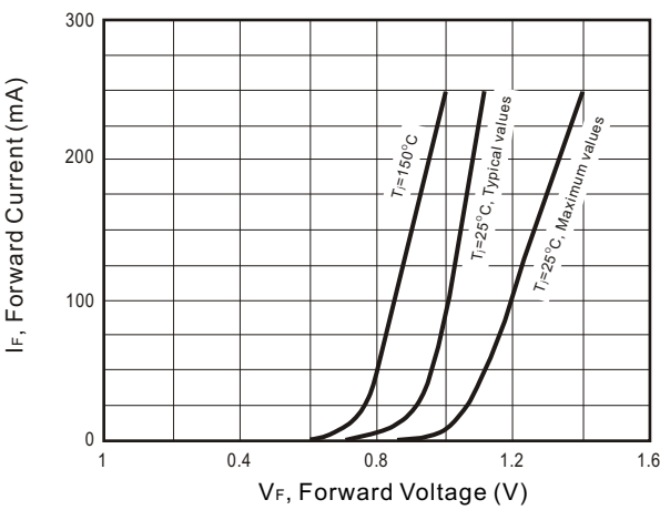
Fig.2 Forward Voltage Characteristics
