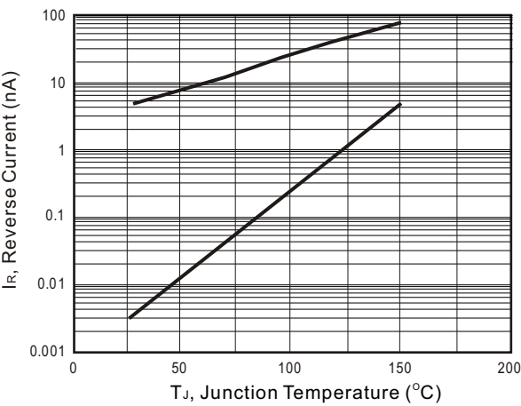
Fig.3 Reverse Characteristics
