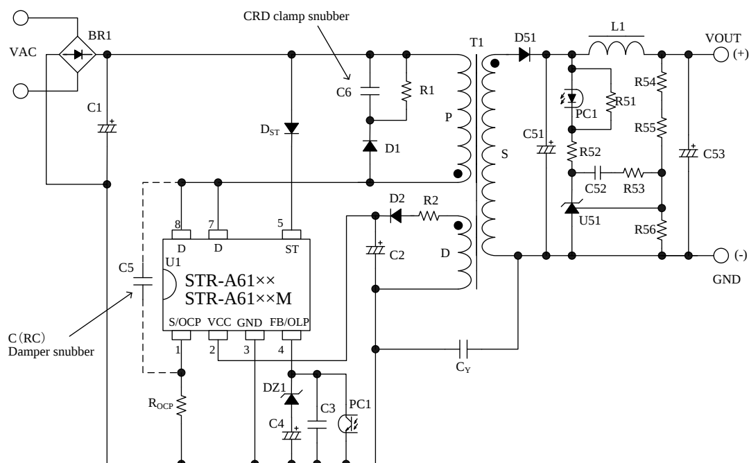
Figure 6-1 Typical application circuit (STR-A61××/ STR-A61××M)
