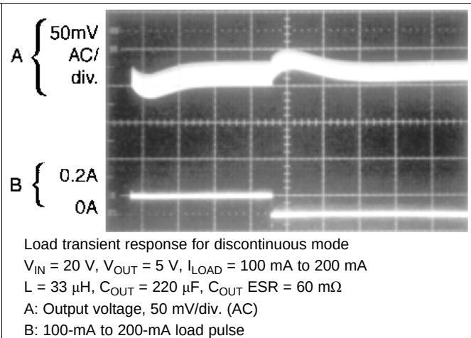
Figure 45. Horizontal Time Base: 200 \mu\text{s}/\text{div}
