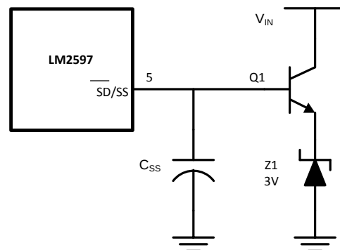
Figure 32. External 3.7-V Soft-Start Clamp
