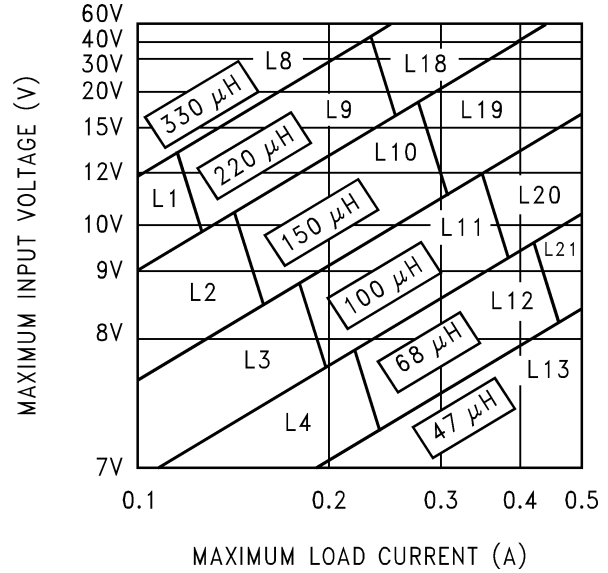
Figure 39. LM2597xx 5-V Version
