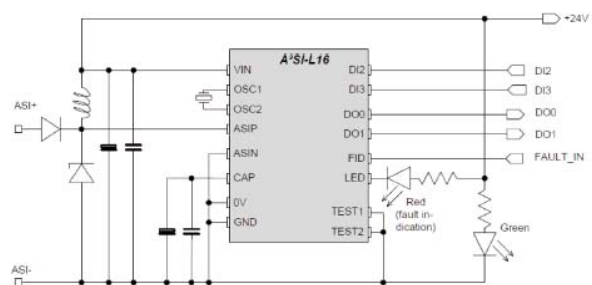
Figure 9-2: Typical application II
