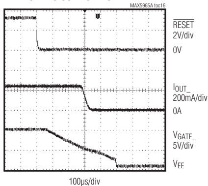
RESET TO OUT TURN-OFF DELAY
