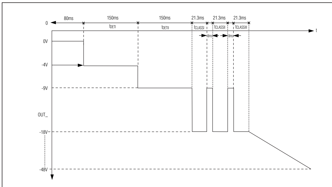
Figure 1b. Detection, 2-Event Classification, and Power-Up Port Sequence
