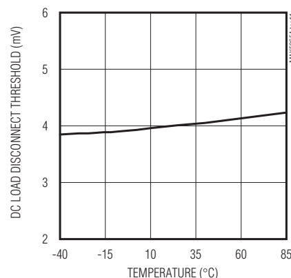
DC LOAD DISCONNECT THRESHOLD vs. TEMPERATURE
