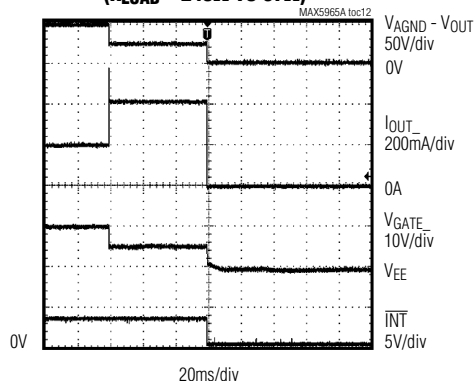
OVERCURRENT TIMEOUT ( R_{LOAD} = 240\Omega TO 57\Omega )
