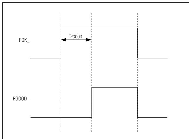
Figure 2. PGOOD_ Timing
