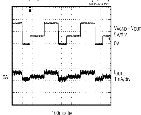
DETECTION WITH INVALID PD (15k \Omega )
