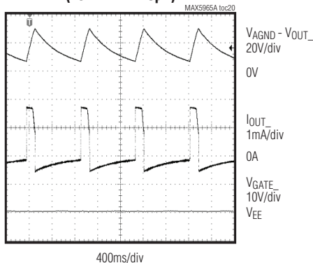
DETECTION WITH INVALID PD (25k \Omega AND 10 \mu F)
