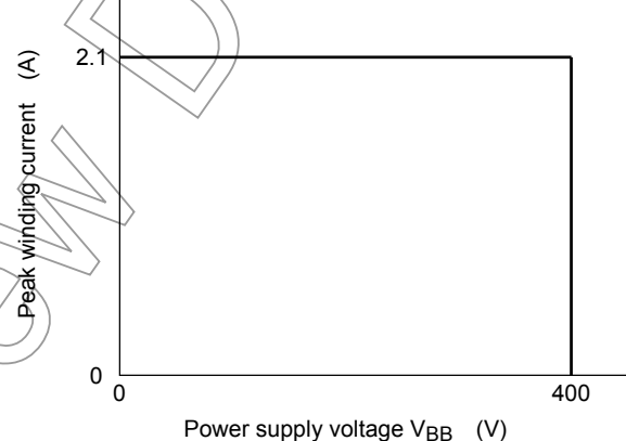
Figure 2 SOA at T_c = 95^{\circ}\text{C}
