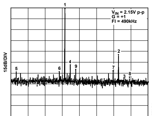
Figure 41. FFT of AD1672 Output Driven by AD823
