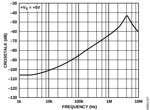
Figure 27. Crosstalk vs. Frequency
