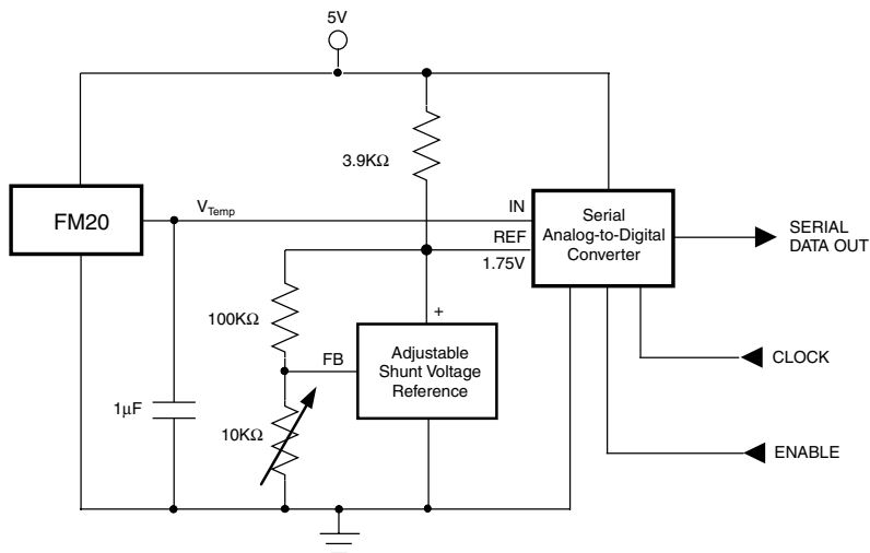
Figure 4. Serial Output Temperature to Digital Converter
