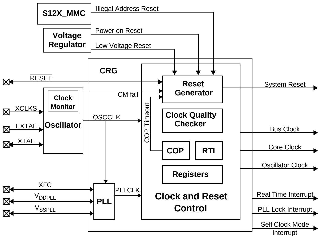
Figure 2-1. CRG Block Diagram
