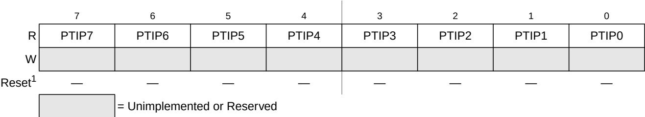
Figure 22-41. Port P Input Register (PTIP)
