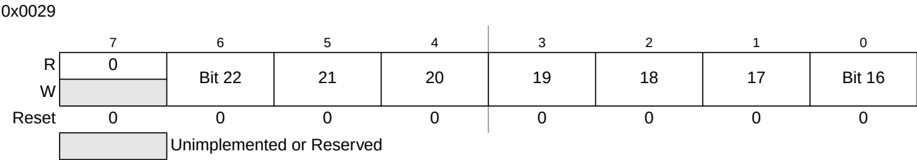
Figure 19-15. Debug Comparator Address High Register (DBGXAH)
