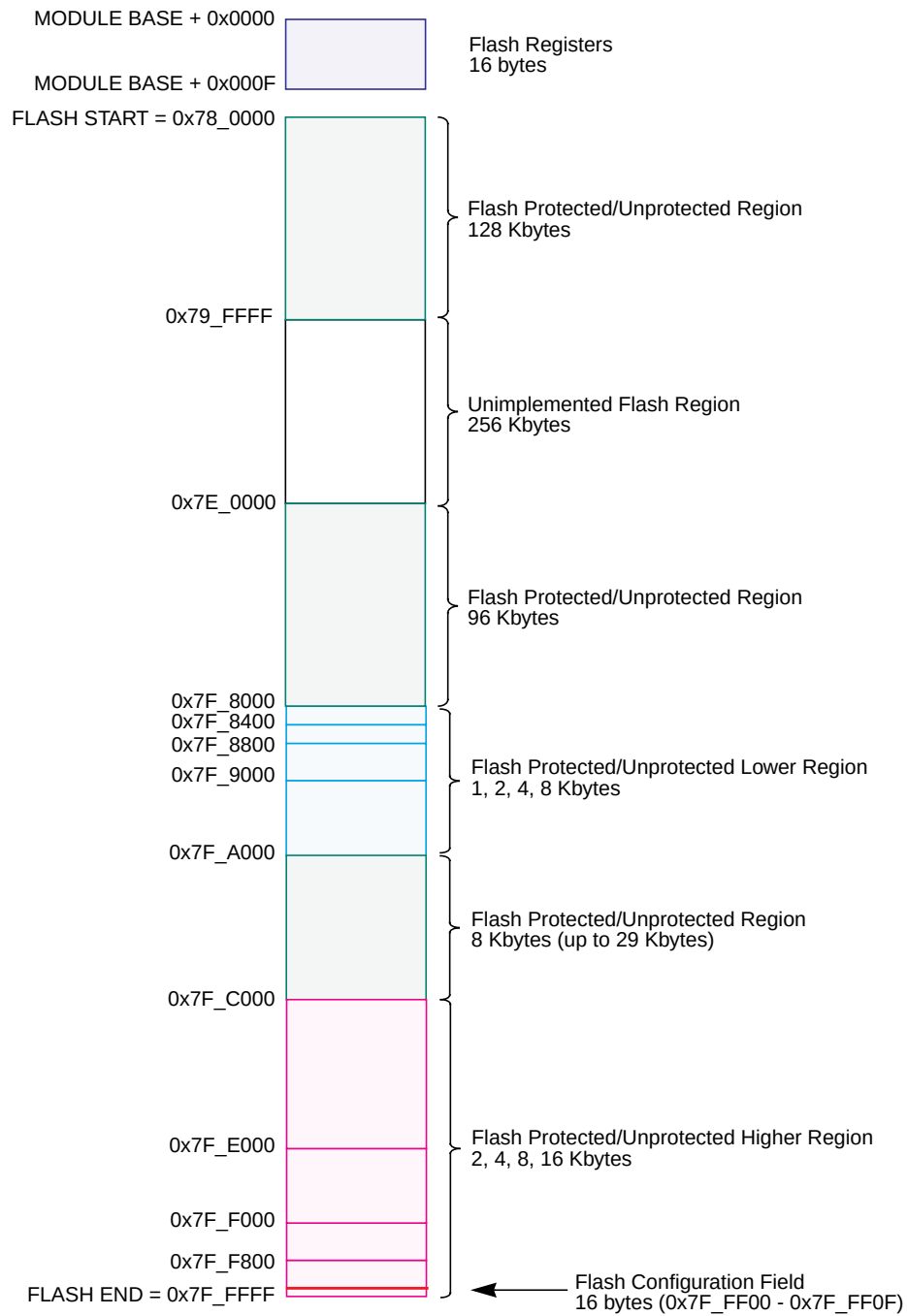
Figure 28-2. Flash Memory Map
