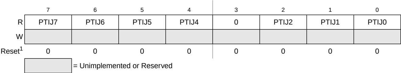
Figure 22-57. Port J Input Register (PTIJ)
