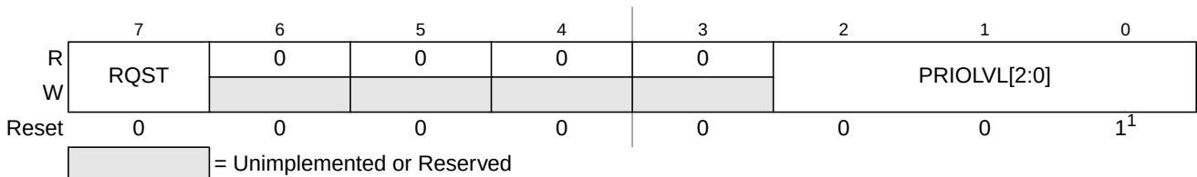
Figure 16-12. Interrupt Request Configuration Data Register 6 (INT_CFDATA6)
