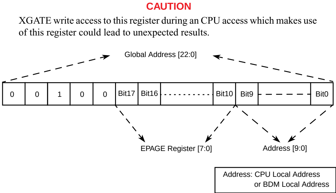
Figure 18-14. EPAGE Address Mapping
