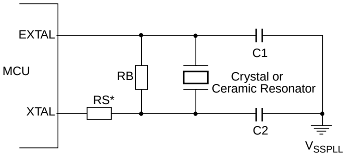
Figure 3-3. Full Swing Pierce Oscillator Connections ( \overline{\text{XCLKS}} = 0 )
