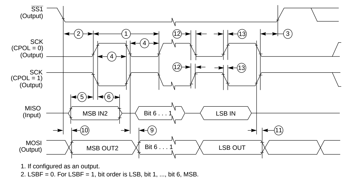
Figure A-6. SPI Master Timing (CPHA = 0)
