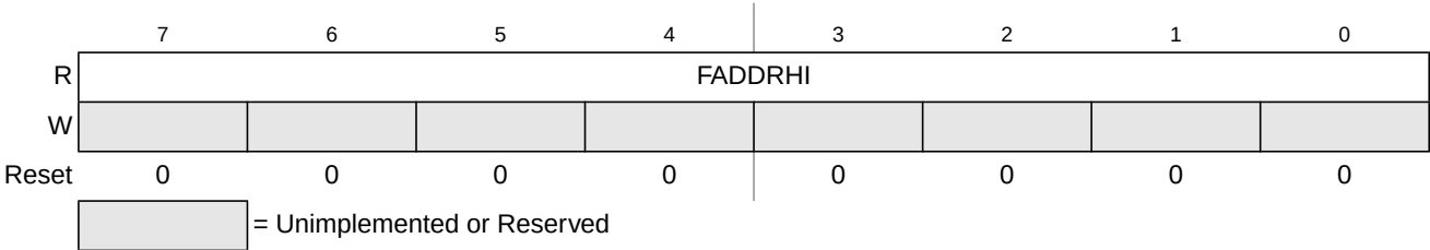
Figure 27-16. Flash Address High Register (FADDRHI)
