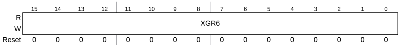
Figure 6-17. XGATE Register 6 (XGR6)
