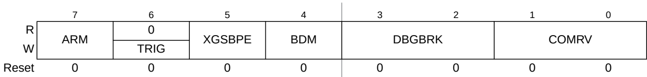
Figure 20-3. Debug Control Register (DBGCR1)
