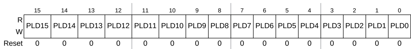
Figure 13-11. PIT Load Register 0 (PITLD0)
