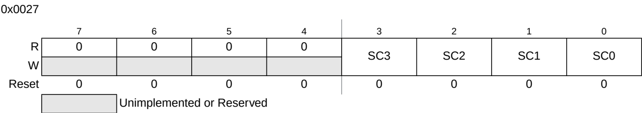
Figure 19-10. Debug State Control Register 1 (DBGSCR1)
