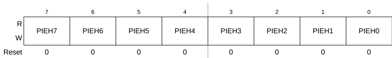
Figure 22-54. Port H Interrupt Enable Register (PIEH)
