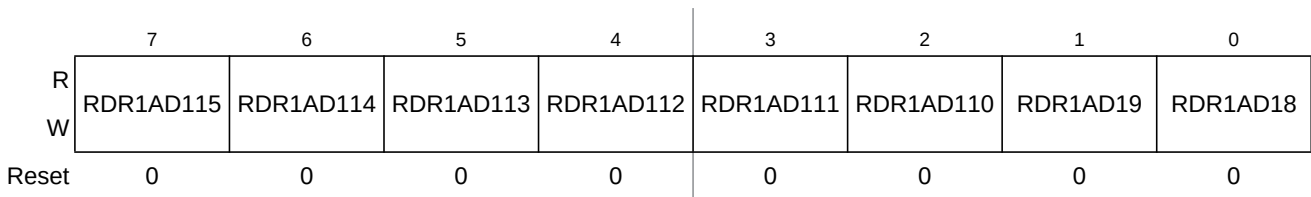
Figure 22-73. Port AD1 Reduced Drive Register 1 (RDR1AD1)
