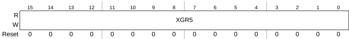
Figure 6-16. XGATE Register 5 (XGR5)
