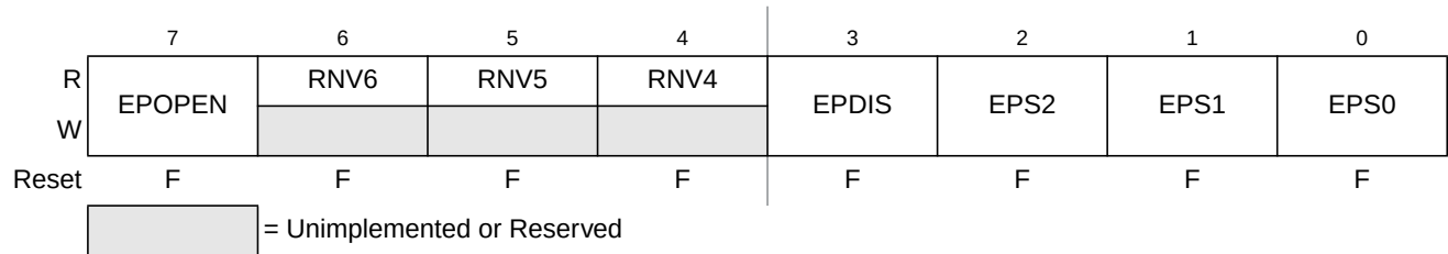
Figure 26-8. EEPROM Protection Register (EPROT)
