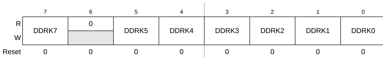
Figure 24-14. Port K Data Direction Register (DDRK)
