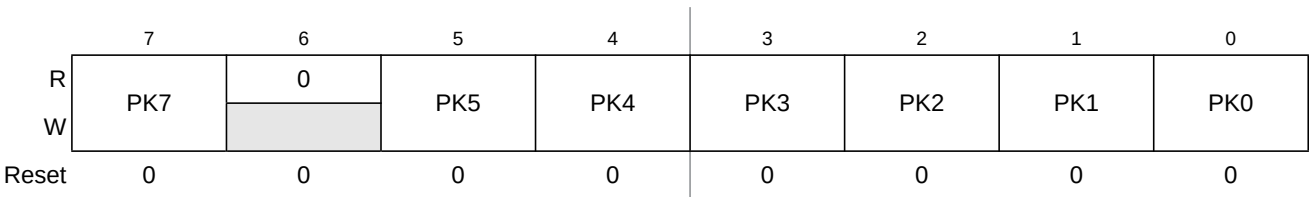
Figure 24-13. Port K Data Register (PORTK)
