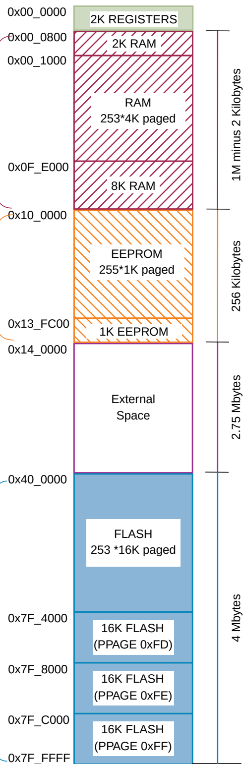
Figure 18-21. Expansion of the Local Address Map
