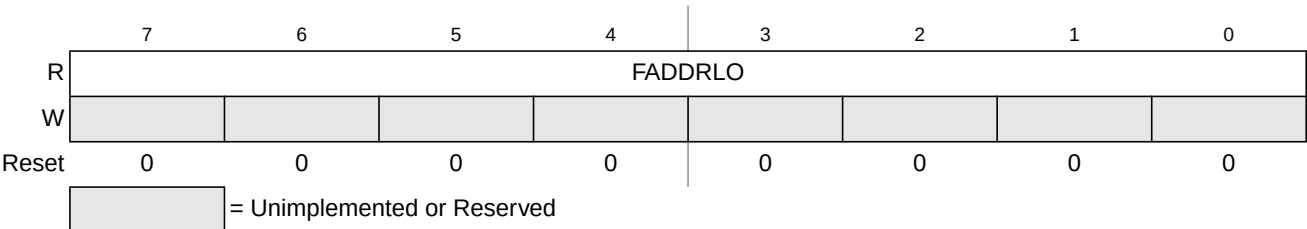
Figure 28-17. Flash Address Low Register (FADDRLO)
