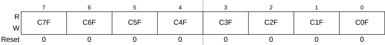
Figure 7-17. Main Timer Interrupt Flag 1 (TFLG1)
