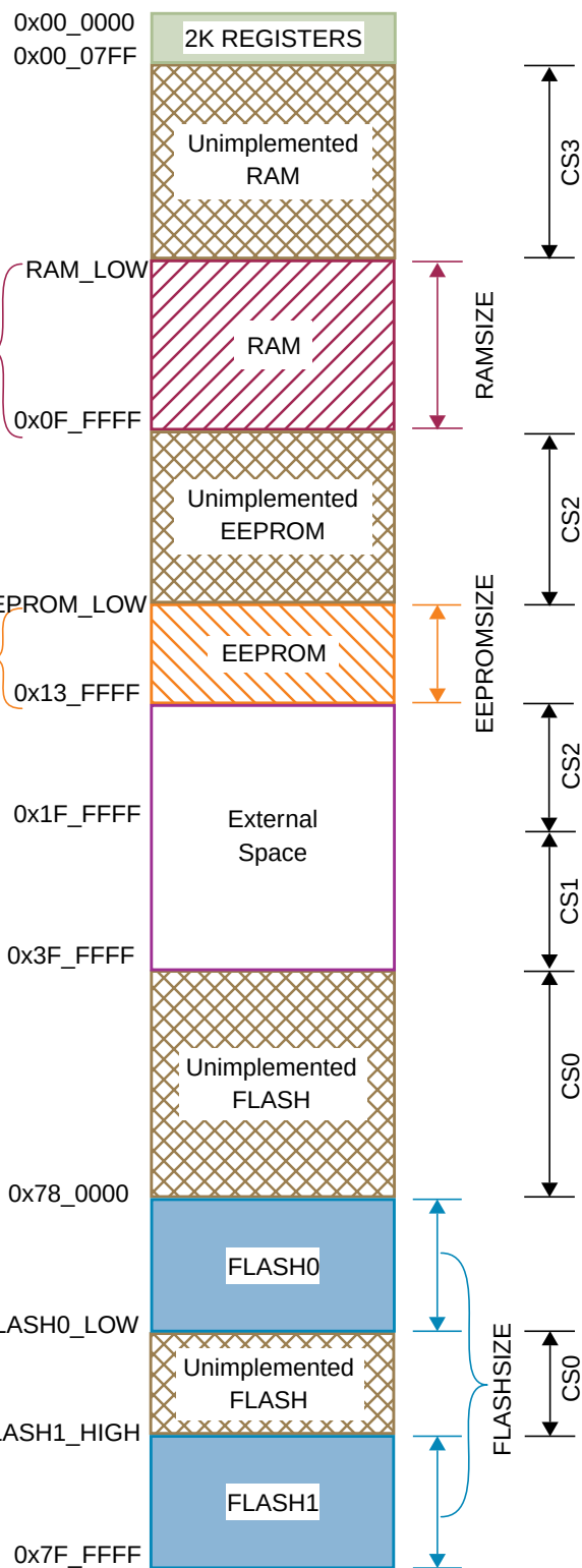
Figure 1-4. S12X CPU & BDM Global Address Mapping
