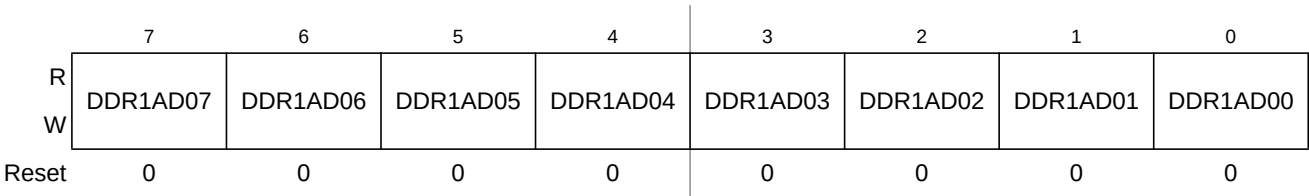
Figure 23-65. Port AD0 Data Direction Register 1 (DDR1AD0)
