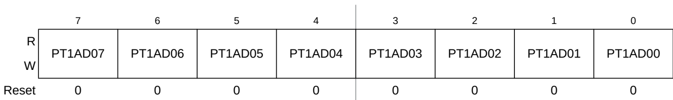
Figure 23-64. Port AD0 Data Register 1 (PT1AD0)
