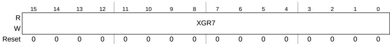
Figure 6-18. XGATE Register 7 (XGR7)
