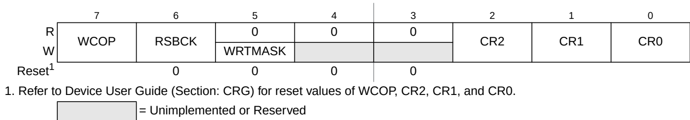
Figure 2-12. CRG COP Control Register (COPCTL)
