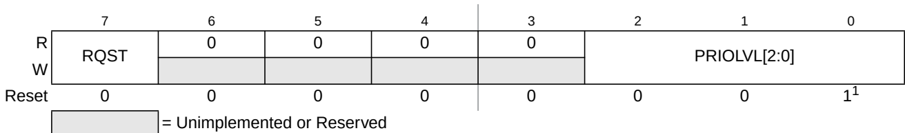
Figure 16-11. Interrupt Request Configuration Data Register 5 (INT_CFDATA5)
