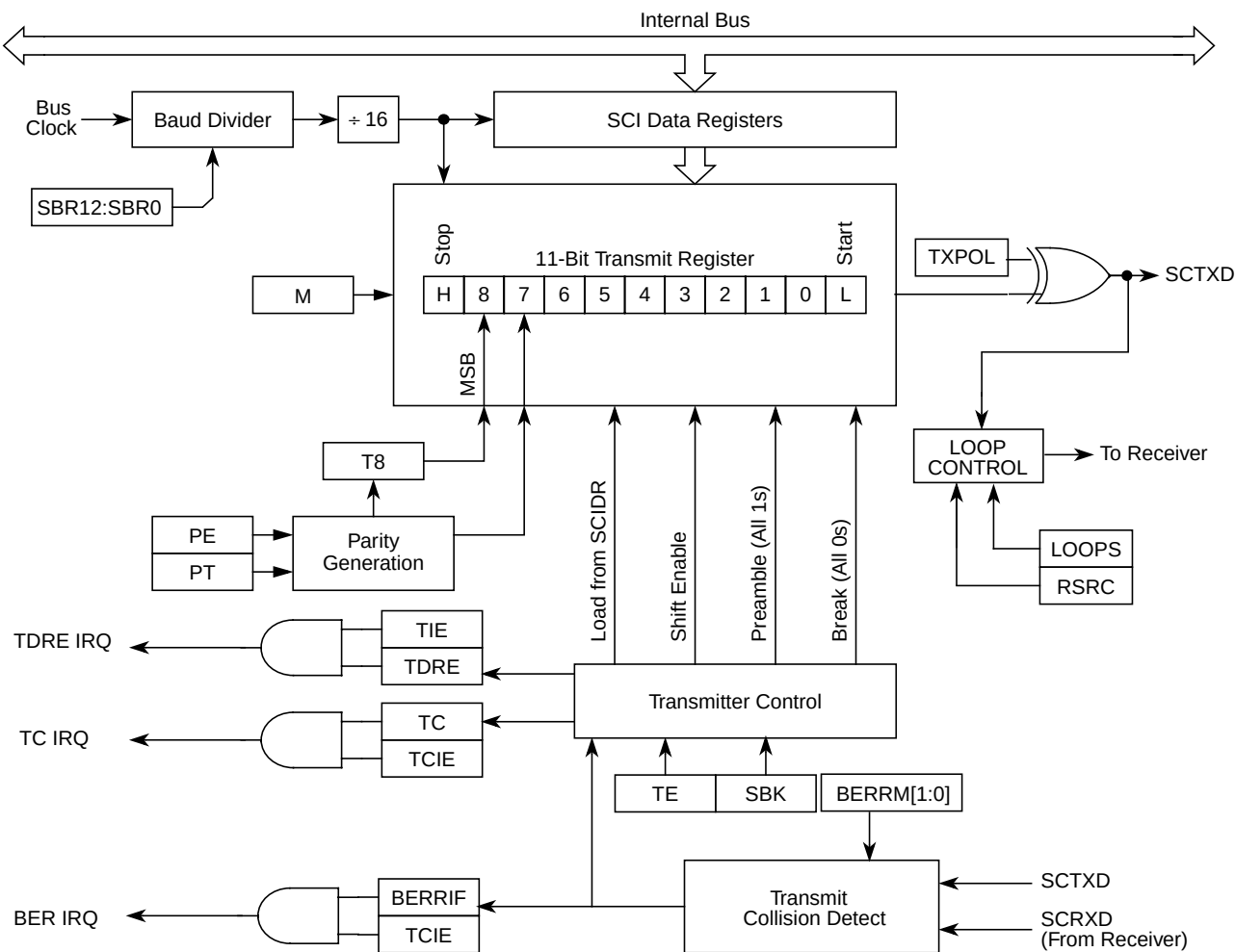
Figure 11-16. Transmitter Block Diagram
