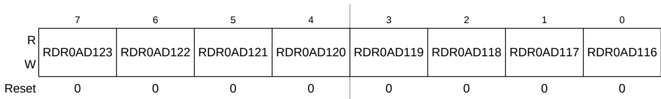
Figure 23-72. Port AD1 Reduced Drive Register 0 (RDR0AD1)
