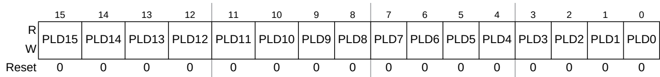
Figure 13-14. PIT Load Register 3 (PITLD3)
