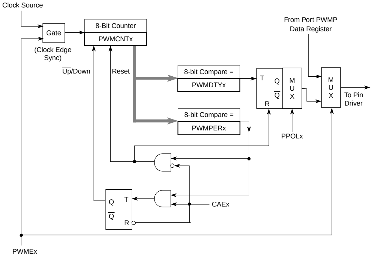
Figure 8-19. PWM Timer Channel Block Diagram
