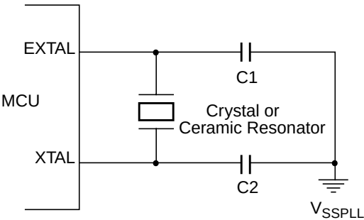
Figure 3-2. Loop Controlled Pierce Oscillator Connections ( \overline{\text{XCLKS}} = 1 )
