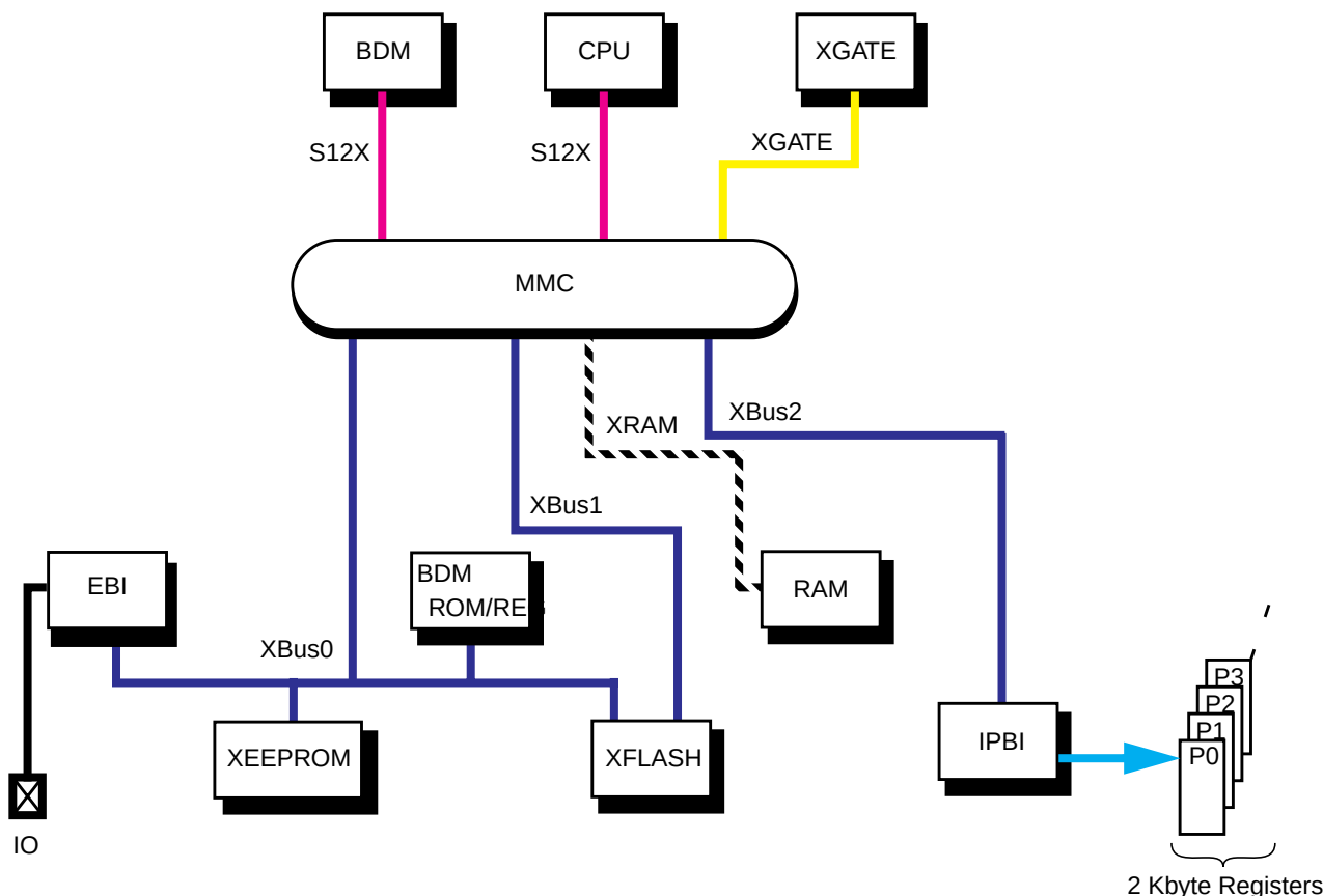
Figure 17-26. S12X Architecture
