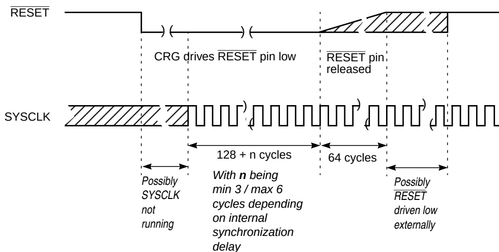
Figure 2-25. RESET Timing
