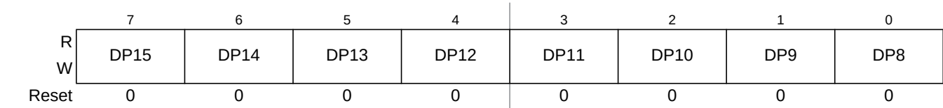
Figure 18-8. Direct Register (DIRECT)
