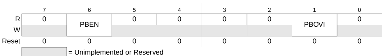
Figure 7-49. 16-Bit Pulse Accumulator B Control Register (PBCTL)
