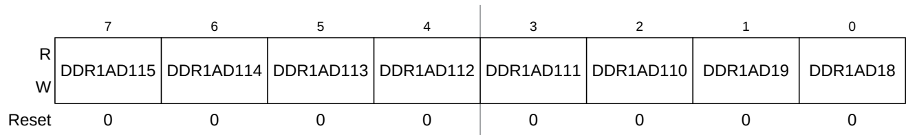
Figure 22-71. Port AD1 Data Direction Register 1 (DDR1AD1)
