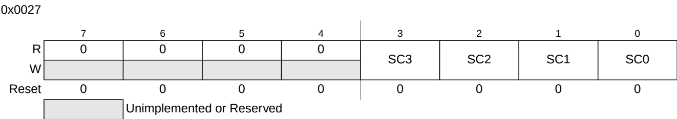
Figure 19-12. Debug State Control Register 3 (DBGSCR3)
