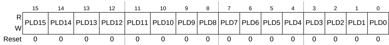
Figure 13-12. PIT Load Register 1 (PITLD1)
