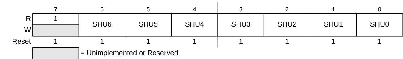
Figure 18-20. RAM Shared Region Upper Boundary Register (RAMSHU)
