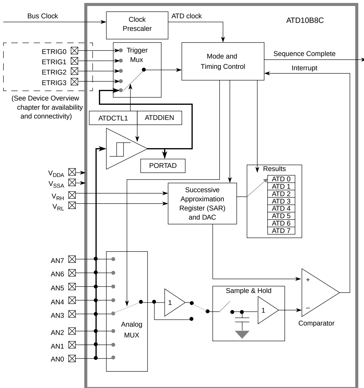
Figure 5-1. ATD Block Diagram
