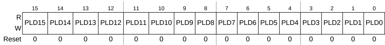
Figure 13-13. PIT Load Register 2 (PITLD2)
