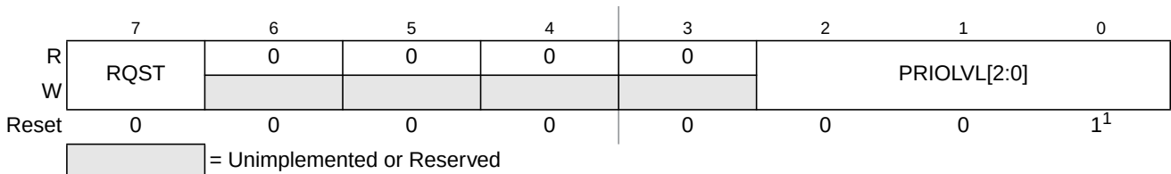
Figure 16-13. Interrupt Request Configuration Data Register 7 (INT_CFDATA7)
