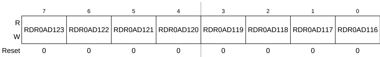
Figure 22-72. Port AD1 Reduced Drive Register 0 (RDR0AD1)
