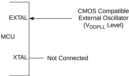
Figure 3-4. External Clock Connections ( \overline{\text{XCLKS}} = 0 )
