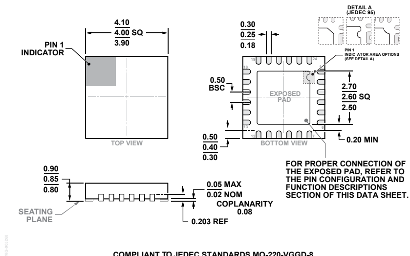
Figure 23. 24-Lead Lead Frame Chip Scale Package [LFCSP] 4 mm × 4 mm Body and 0.85 mm Package Height (HCP-24-3)
