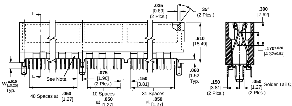
Section L-L
