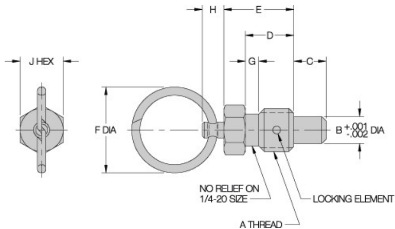
PULL RING, NON-LOCKING TYPE — STEEL (USA)
