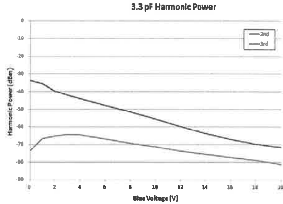
Figure 3. Harmonic Power*
