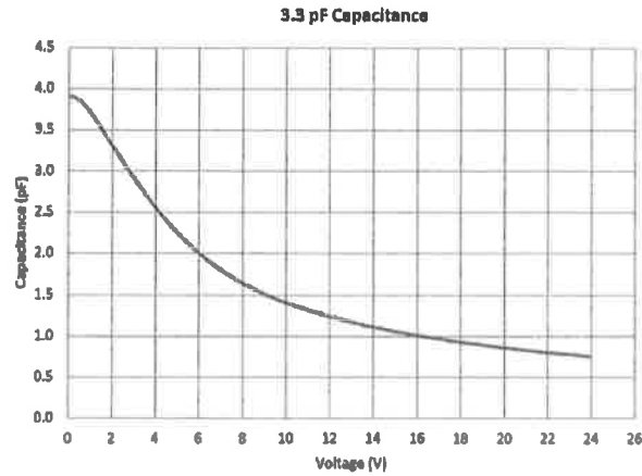
Figure 2. Capacitance
