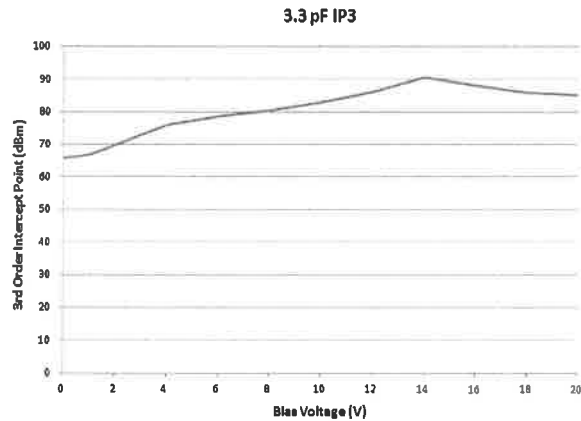
Figure 4. IP3*
