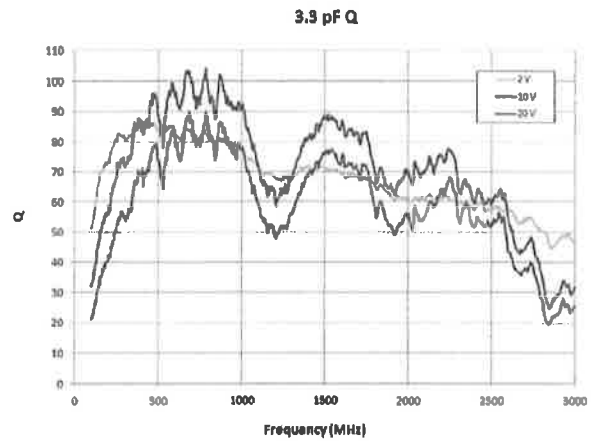
Figure 5. Q*
