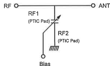
Figure 7. PTIC Orientation Functional Block Diagram
