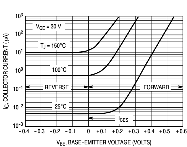
Figure 12. Collector Cut-Off Region
