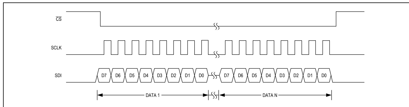
Figure 2. SPI Format
