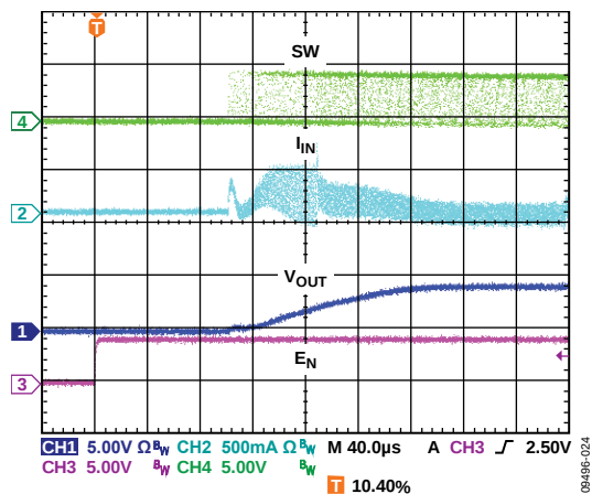
Figure 28. Startup, V_{OUT} = 0.8\text{ V} , I_{OUT} = 10\text{ mA}
