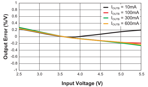
Buck Line Regulation ( V_{OUTB} = 1.2V , L = 2.2\mu H )
