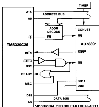
Figure 17. AD7880-TMS320C25 Interface
