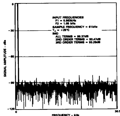
Figure 14. IMD Plot
