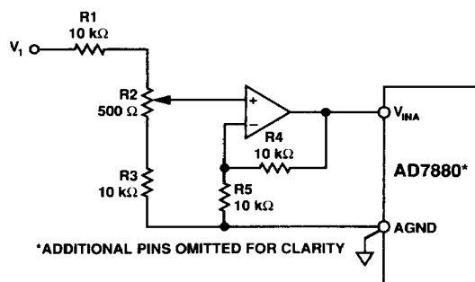
Figure 11. Offset and Full-Scale Adjust Circuit
