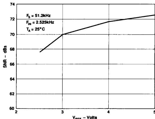
Figure 3. SNR Versus V_{\text{REF}}
