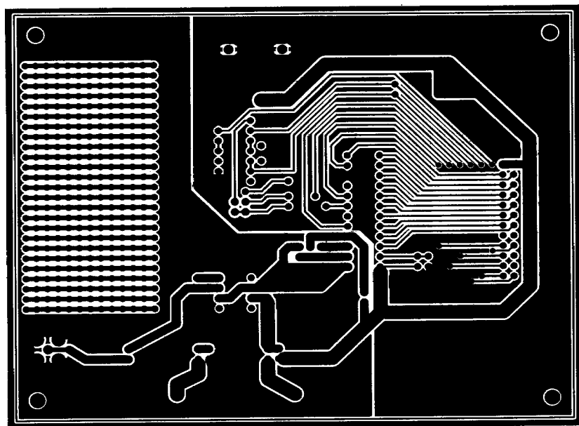
Figure 27. PCB Solder Side Layout for Figure 24
