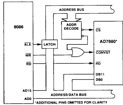
Figure 19. AD7880-8086 Interface
