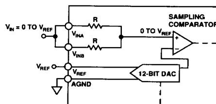
Figure 5. 0 to V_{\text{REF}} Unipolar Input Configuration
