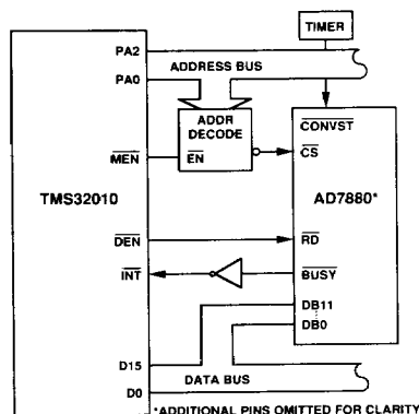
Figure 16. AD7880-TMS32010 Interface
