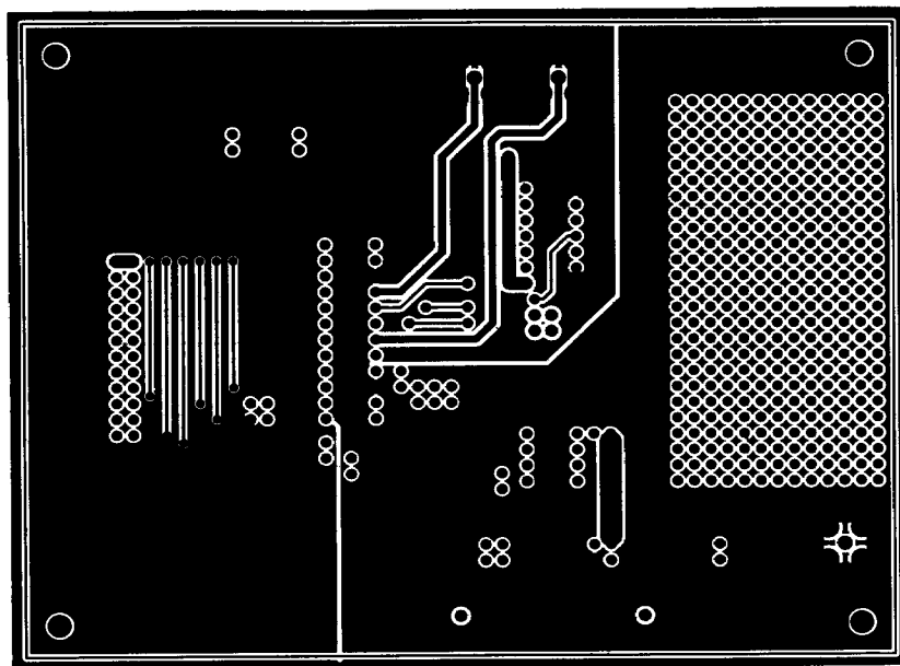
Figure 26. PCB Component Side Layout for Figure 24
