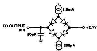
Figure 2. Load Circuit for Access and Relinquish Time
