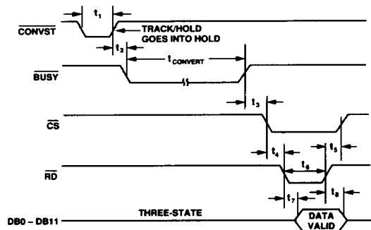
Figure 1. Timing Diagram
