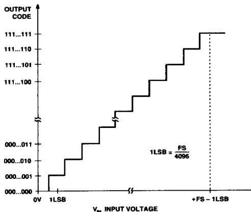
Figure 8. AD7880 Unipolar Transfer Characteristic
