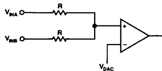
Figure 4. AD7880 Input Circuit
