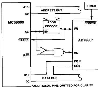
Figure 18. AD7880-MC68000 Interface
