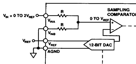
Figure 6. 0 to 2 V_{\text{REF}} Unipolar Input Configuration
