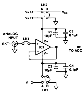
Figure 21. Analog Input Buffering
