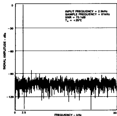
Figure 12. FFT Plot
