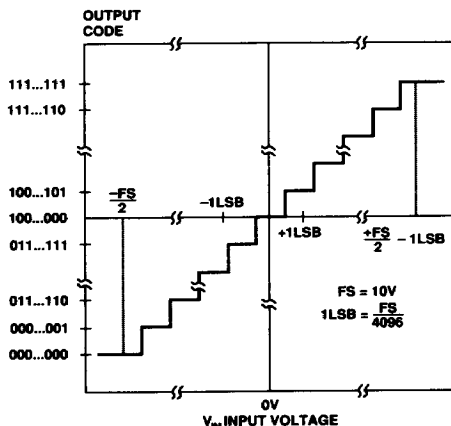
Figure 9. AD7880 Bipolar Transfer Characteristic
