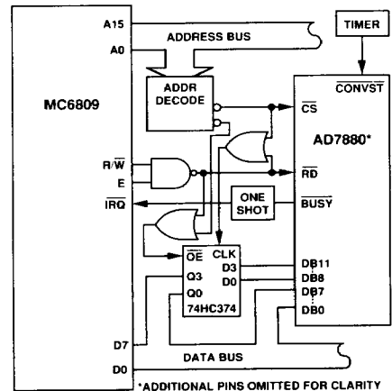
Figure 20. AD7880-6809 Interface
