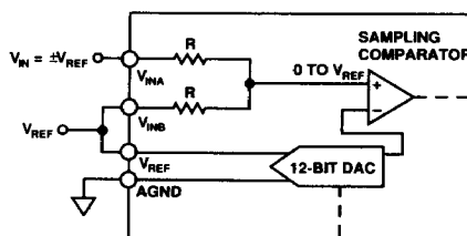
Figure 7. \pm V_{\text{REF}} Bipolar Input Configuration
