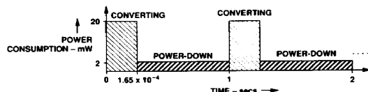
Figure 22. Power Consumption for Normal Operation and Power-Down Operation vs. Time
