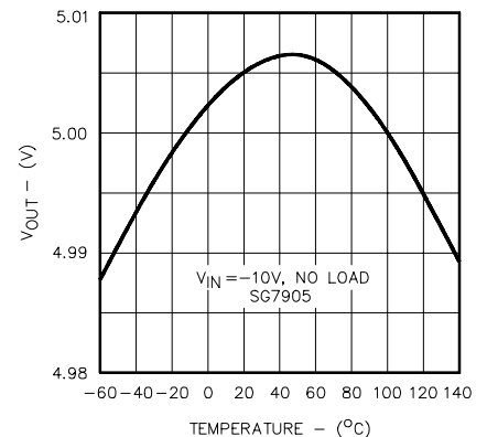
FIGURE 3. TEMPERATURE COEFFICIENT
