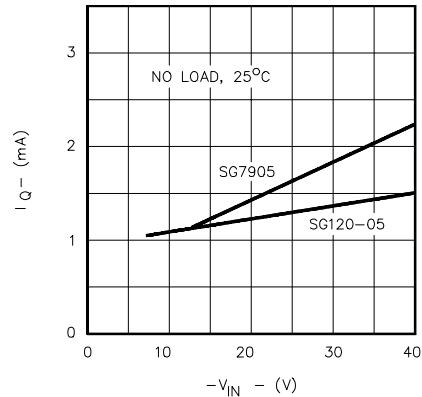
FIGURE 5. QUIESCENT CURRENT VS. V_{IN}
