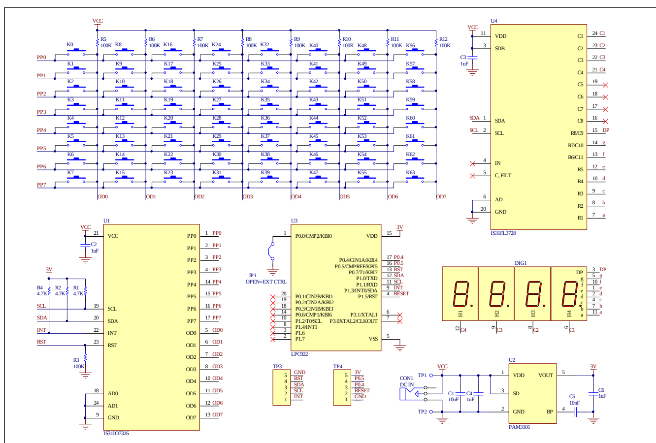
Figure 2:IS31/O7326 Application Schematic
