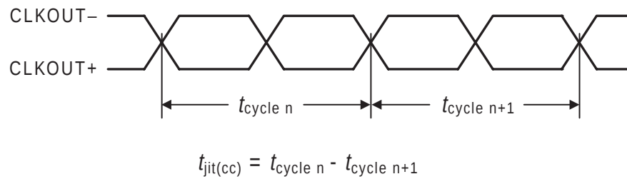
Figure 6. Cycle-to-Cycle Jitter
