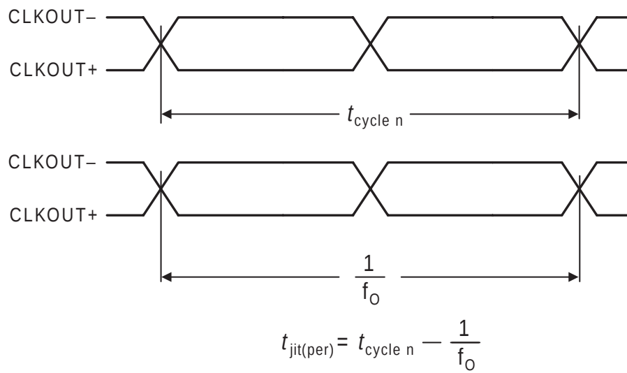
Figure 7. Period Jitter
