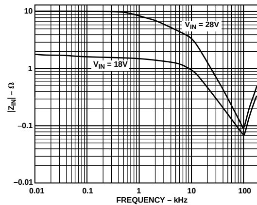
Figure 12. Incremental Input Impedance (Magnitude)
