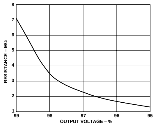
Figure 18. External Resistor Value for Reducing Output Voltage
