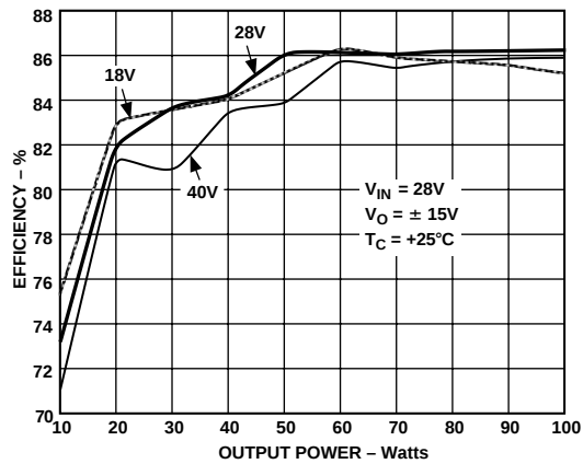
Figure 2. Efficiency vs. Line and Load at +25°C (ADDC02815DA)
