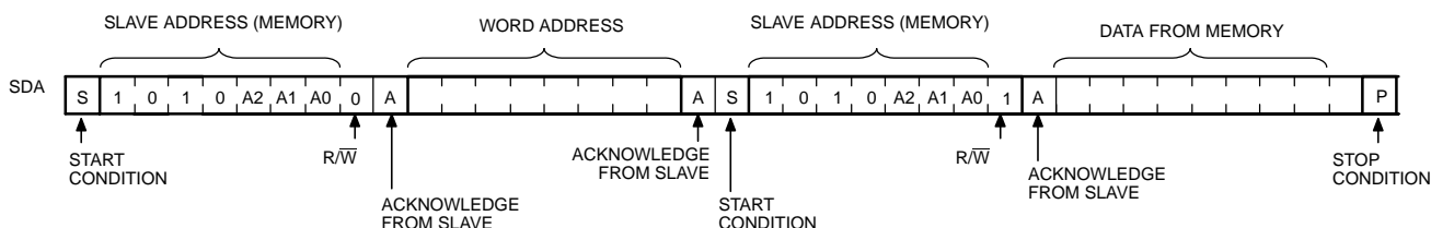
Figure 12. Random Read
