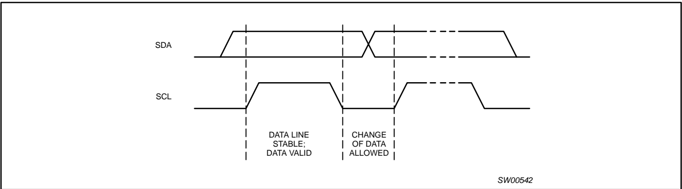
Figure 14. Bit transfer
