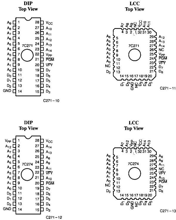
Figure 1. Programming Pinouts
