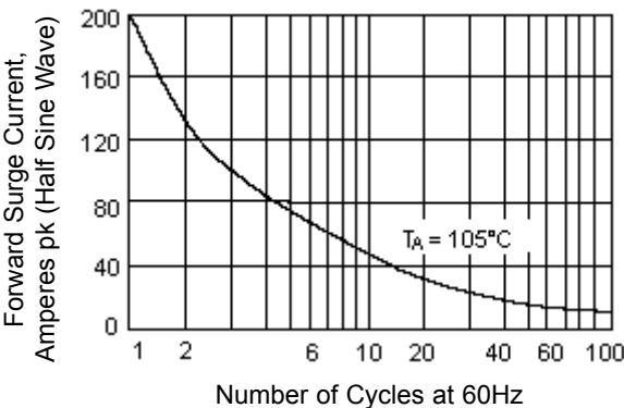
Figure 4 - Non-Recurrent Surge Rating
