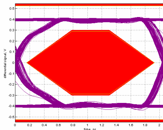
Figure 3 - USB Eye Pattern with RClamp1644T
