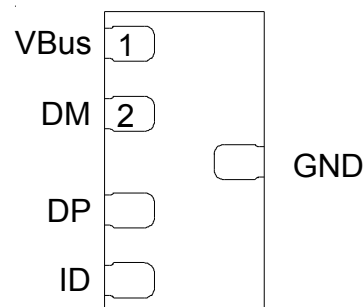
Figure 1 - Pin Configuration (Top View)
