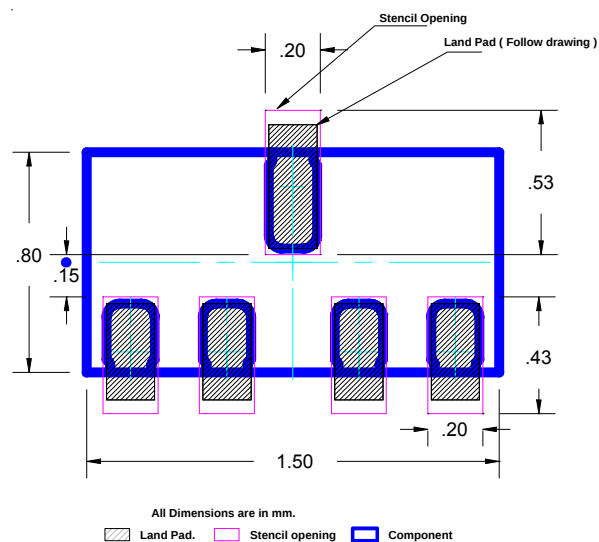
Figure 4 - Recommended Mounting Pattern
