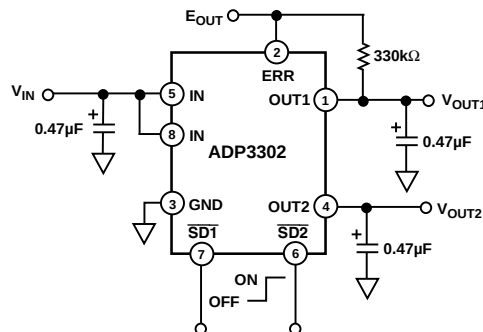
Figure 1. Application Circuit
