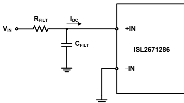
FIGURE 31. INPUT FILTERING
