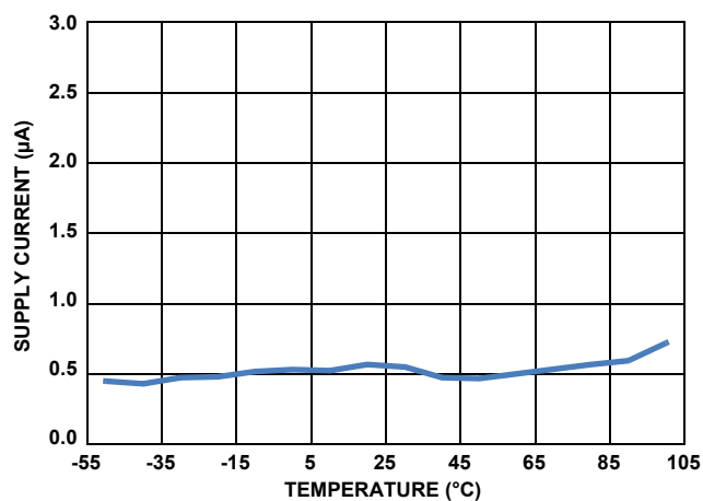
FIGURE 21. POWER-DOWN SUPPLY CURRENT vs TEMPERATURE
