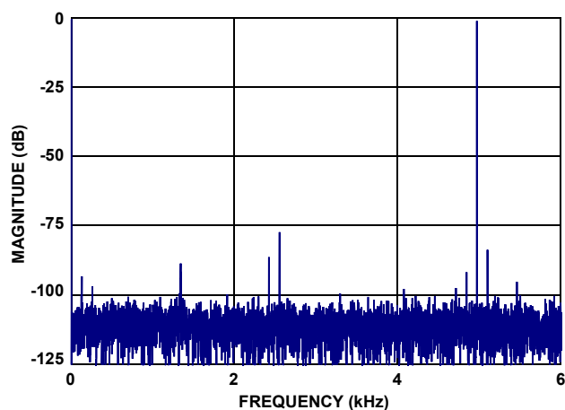
FIGURE 18. 4096 POINT FFT
