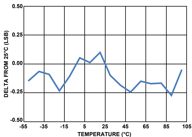
FIGURE 20. CHANGE IN GAIN vs TEMPERATURE
