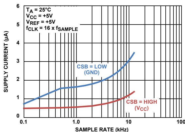
FIGURE 30. SHUTDOWN CURRENT vs SAMPLE RATE
