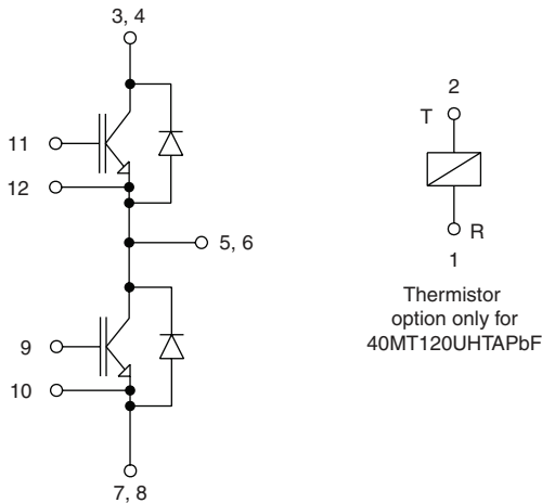
Fig. 25 - Electrical diagram
