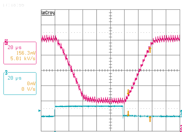
FIGURE 44. GPU MODE VID TRANSITION, DPRSLPVR = 0, I_O = 2A , V_{ID} = 1.2375V/1.0375V , Ch2: V_O , Ch3: VID4
