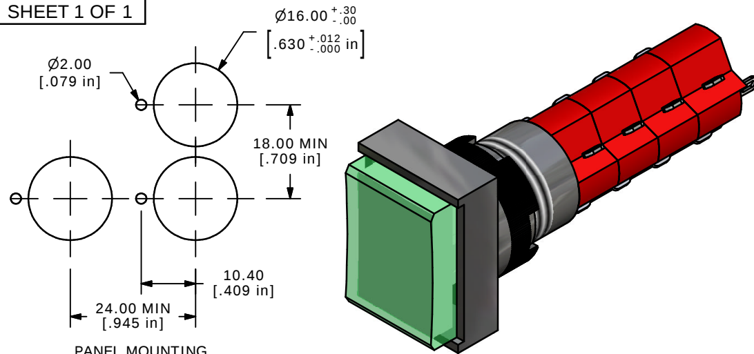
PANEL MOUNTING
