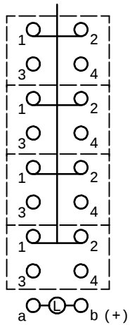
CONTACT CONFIGURATION
