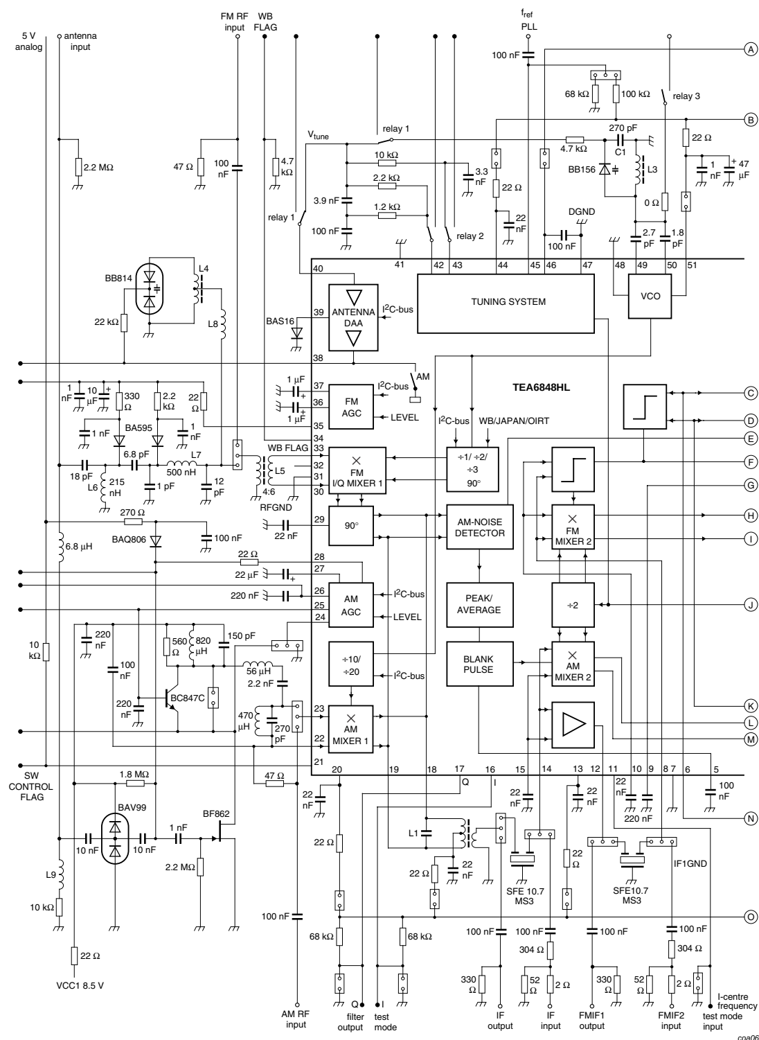
Fig 12. Test circuit (continued in Figure 13 )
