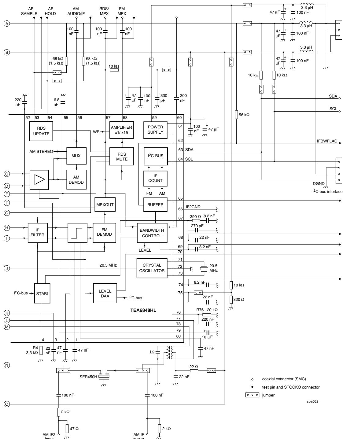
Fig 13. Test circuit (continued from Figure 12)
