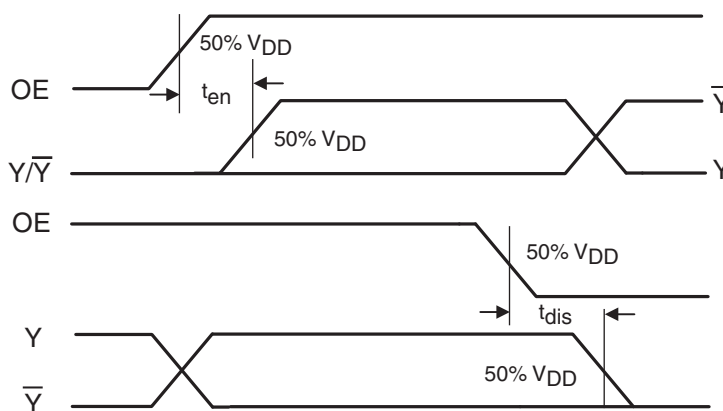
Figure 11. Time Delay Between Output Enable (OE) and Clock Output ( \bar{Y} , Y)
