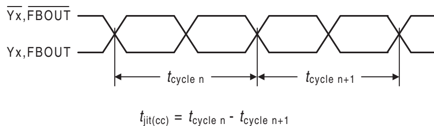
Figure 4. Cycle-to-Cycle Jitter
