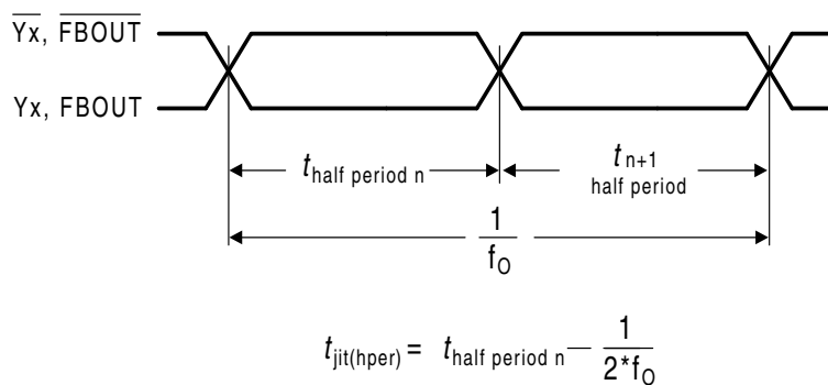
Figure 8. Half-Period Jitter
